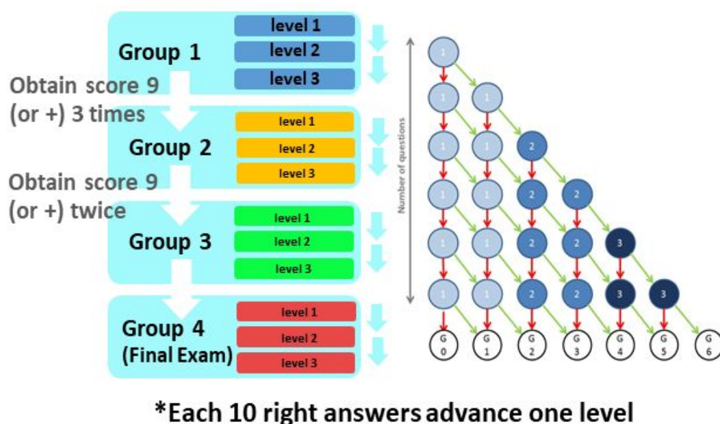
Fig. 1. Representation of the proposed sequential adaptive test model. On the left it is shown the 4-group
